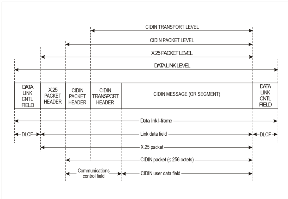
Figure 8-2. CIDIN terminology
