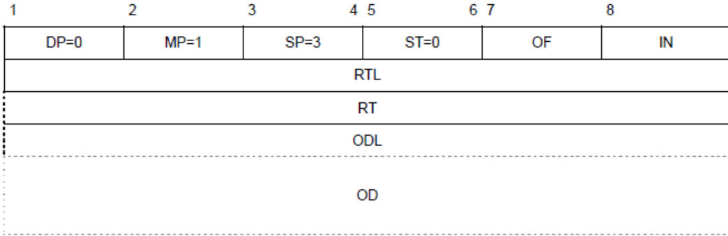
Figure 5-19. ROUTE packet
