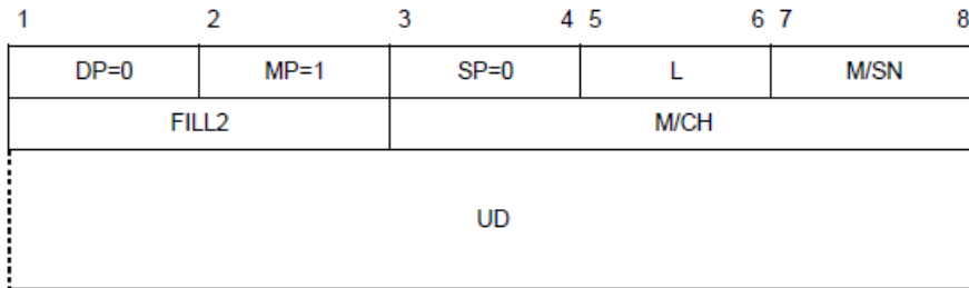
Figure 5-22. LONG FORM MSP packet
