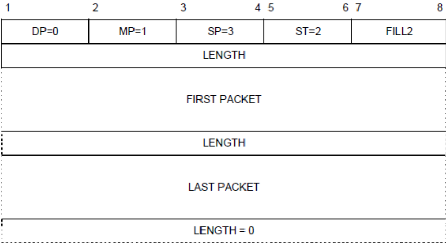
Figure 5-20. MULTIPLEX packet
