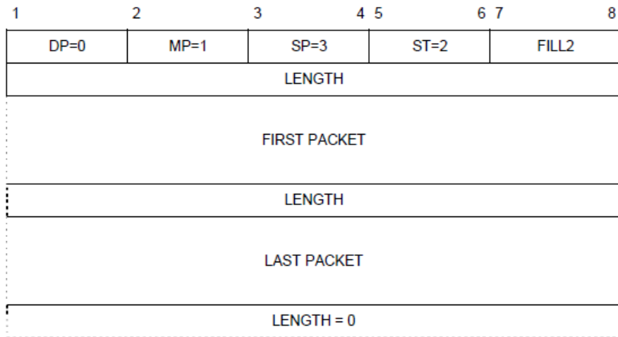
Figure 5-20. MULTIPLEX packet
